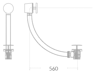
Bath Waste with Overflow Click Clack Waste
