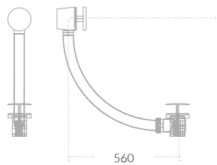
Bath Waste with Overflow Click Clack Waste
